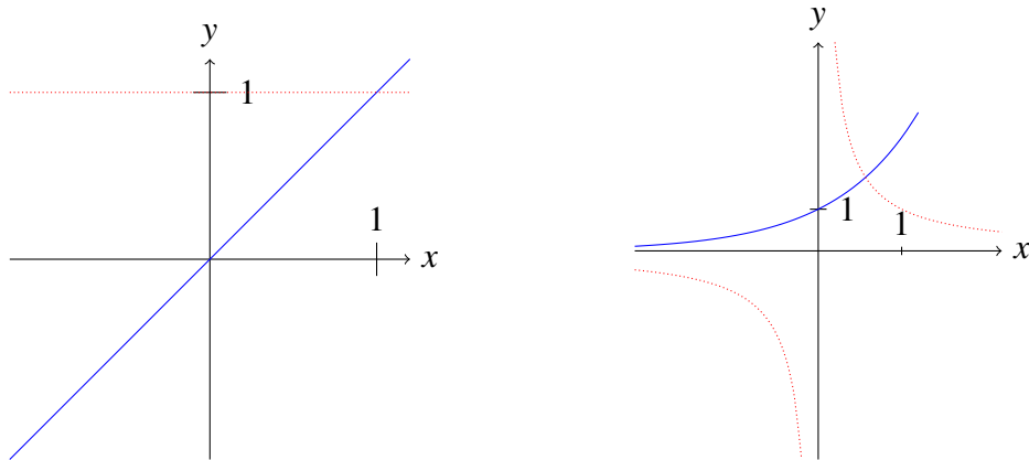
FIGURE 6 – f_1(x) = 1 , f_2(x) = x , f_3(x) = e^x et f_4(x) = \frac{1}{x}
